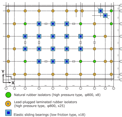
Fig. 9 Plan of seismic isolation components
