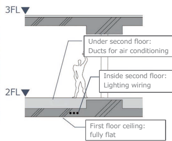
Fig. 7 Flat slab system consistent with M&E system
