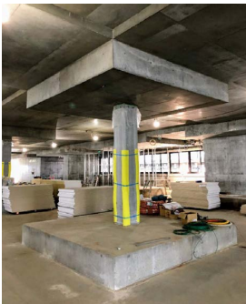
Fig. 5 Flat slab with inverted capital
