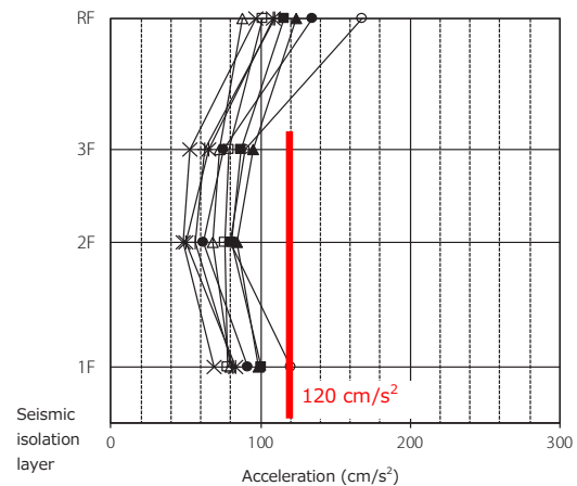
Fig. 10 Example of maximum response values
